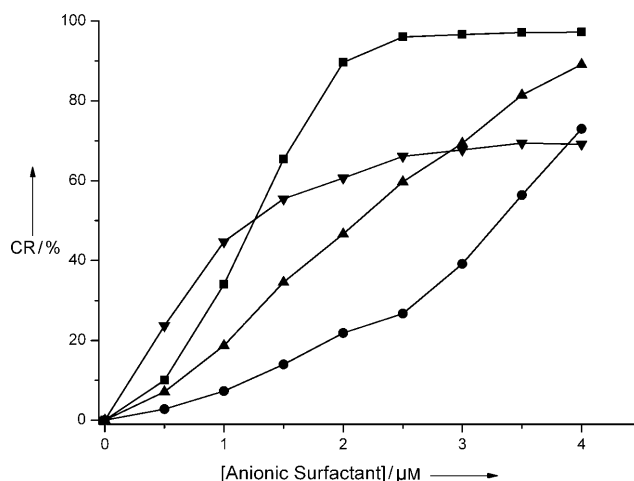
Figure 6. Quantitative colorimetric response of polymer 2 (10 \mu\text{M} ) in the presence of various concentration anionic surfactants in HEPES buffer (20 mM, pH 7.4). ■ SDS, ● SDC, ▲ SDP, ▼ SDBS.
